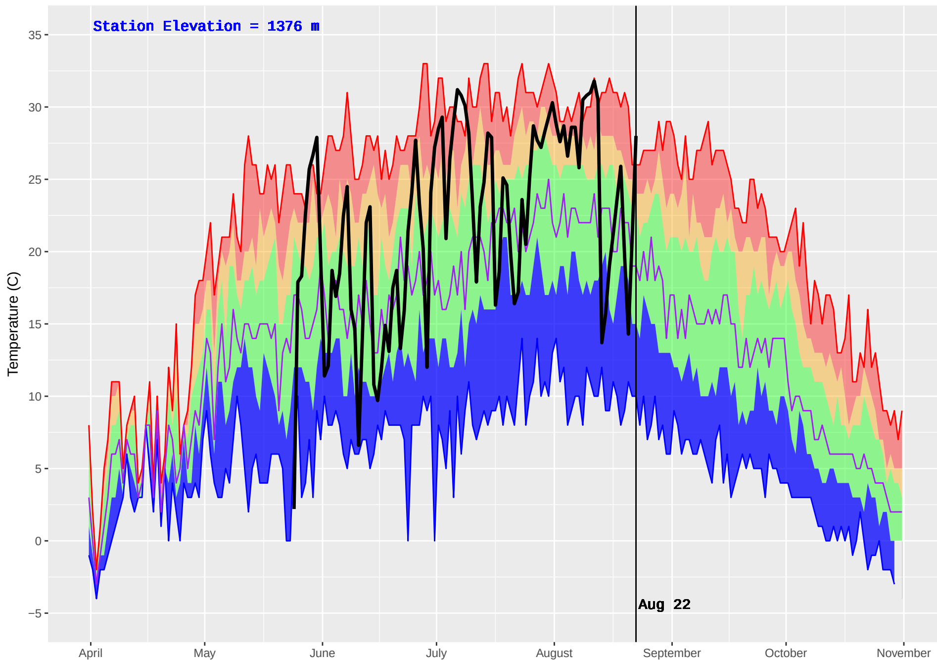
DUNCAN (385) : Historical (1981–2016) and Current (2017) Noon Temperature
